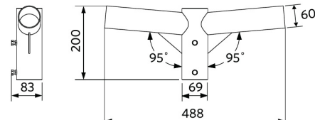
LEDStreetlight Pole-Top-60-Adapter-2x60
