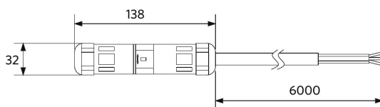
LEDStreet-SE-ExtensionCable
