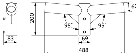
LEDStreetlight Pole-Top-60-Adapter-2x60
