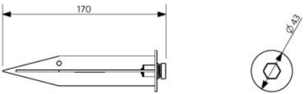
LEDflood-E-Re150-Spike
