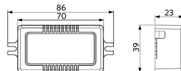
LEDspotRA-Ava-E2 Driver
