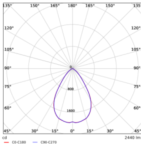
LEDDownlightRc-P-HG R200-23W
